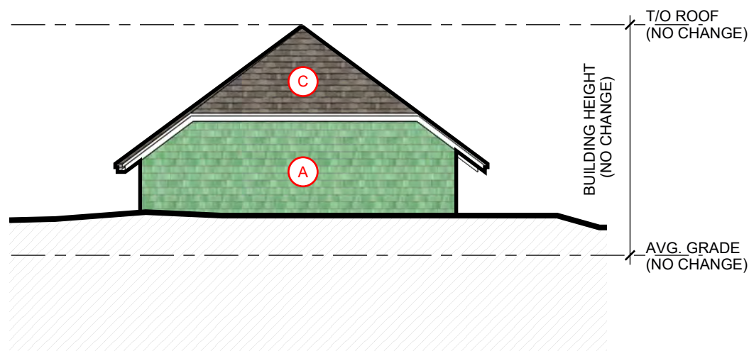
NORTH ELEVATION
