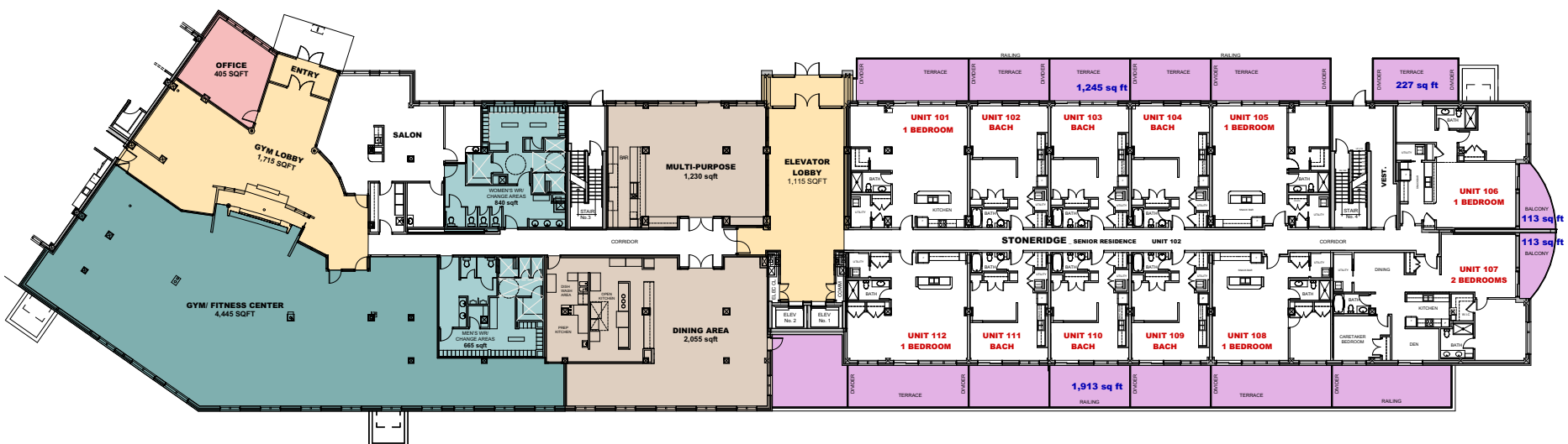
LEVEL 1 _ GROUND FLOOR (TOTAL BALCONY / TERRACE AREA : 3,611 SQFT.)
