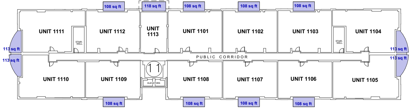
LEVEL 11 (TOTAL BALCONY AREA : 1,431 SQFT.)
