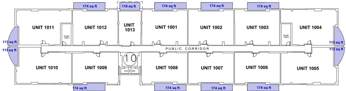
LEVEL 10 (TOTAL BALCONY AREA : 1,957 SQFT.)
