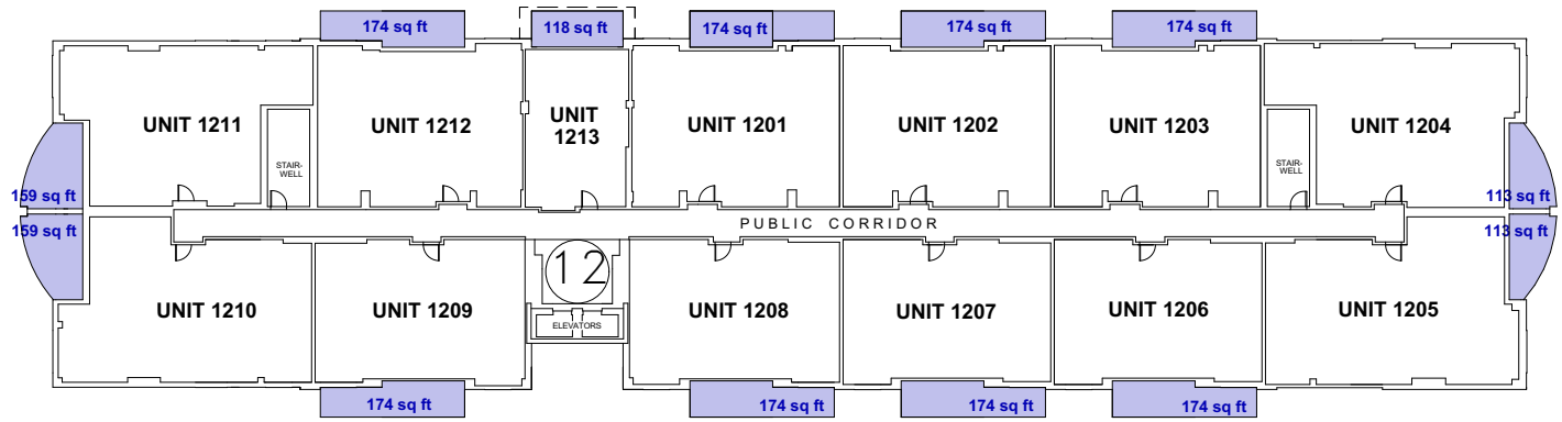
LEVEL 12 (TOTAL BALCONY AREA : 2,049 SQFT.)
