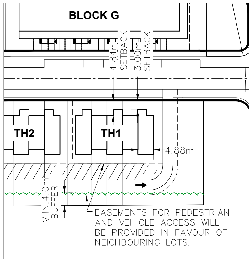
2 TOWNHOUSE DETAILS Scale: 1:750
