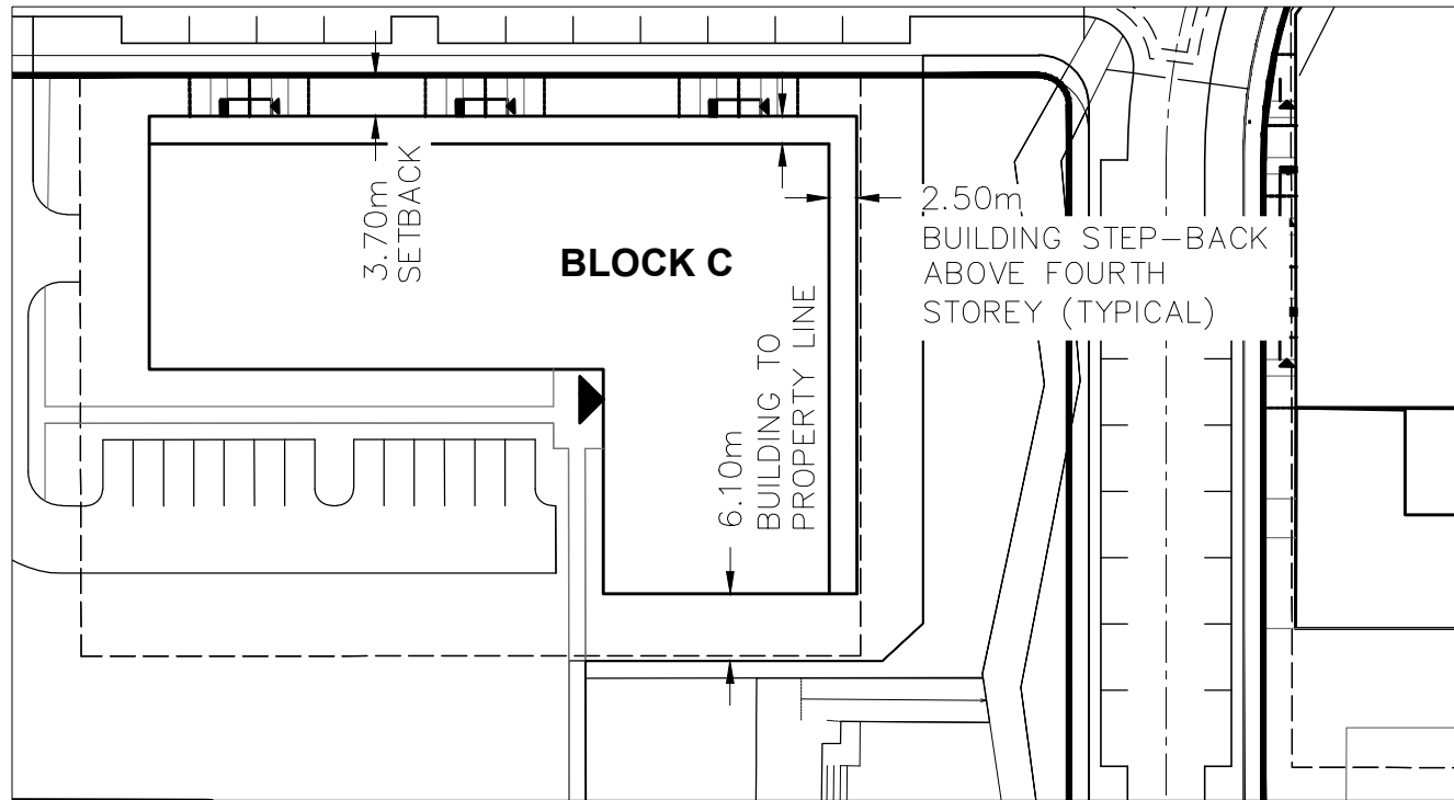
1 BUILDING DETAILS 1 Scale: 1:750
