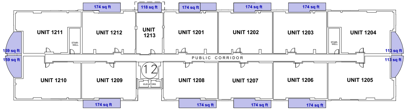
LEVEL 12 (TOTAL BALCONY AREA : 2,049 SQFT.)
