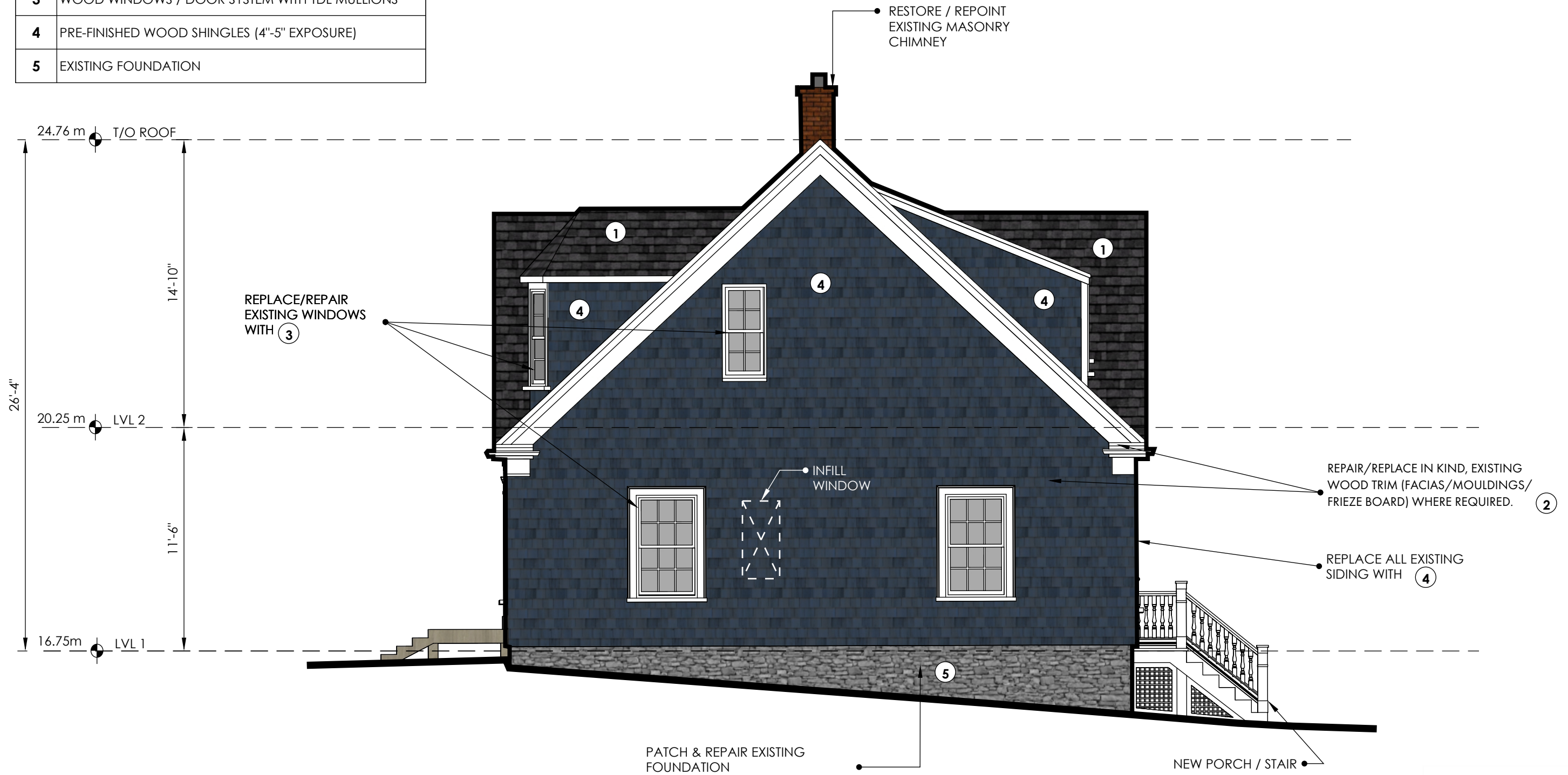
WEST ELEVATION
