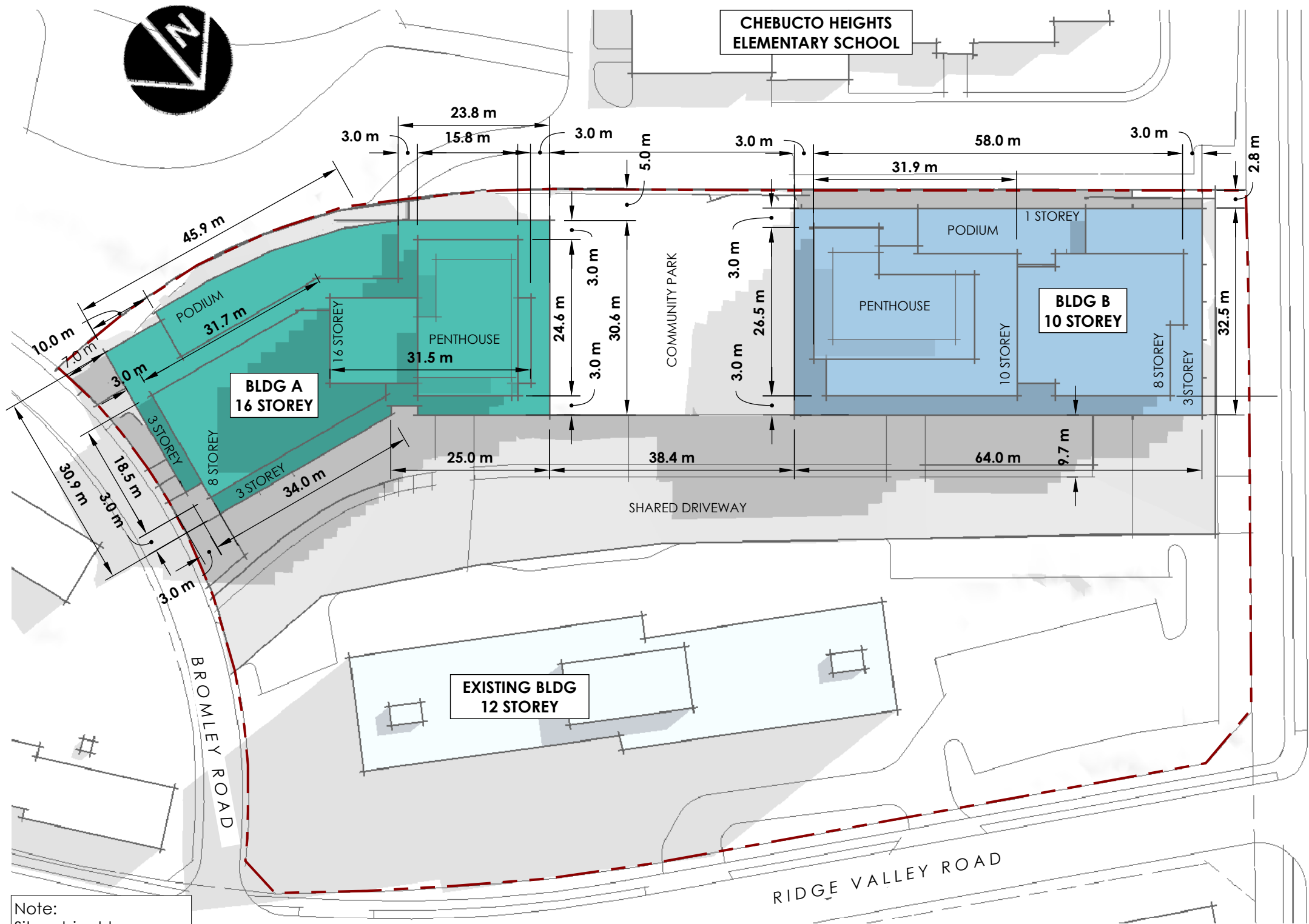
Plan View
