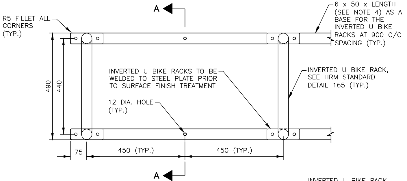
PLAN VIEW
