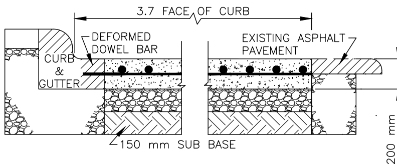
TRANSVERSE SECTION
