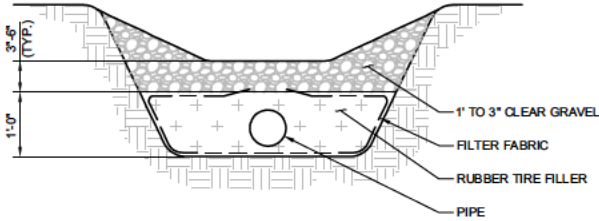
PROPOSED DRAINAGE SWALE DETAIL
