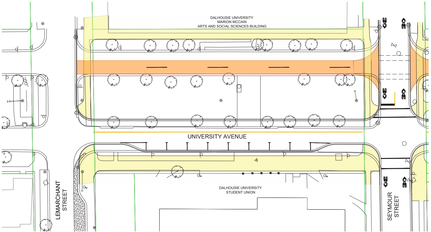
FUNCTIONAL DESIGN CONCEPT 2C Two-Way Bikeway North of Median
