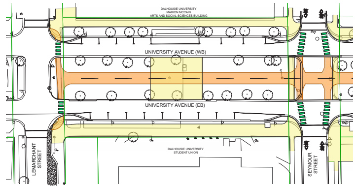
FUNCTIONAL DESIGN - CONCEPT 2B
