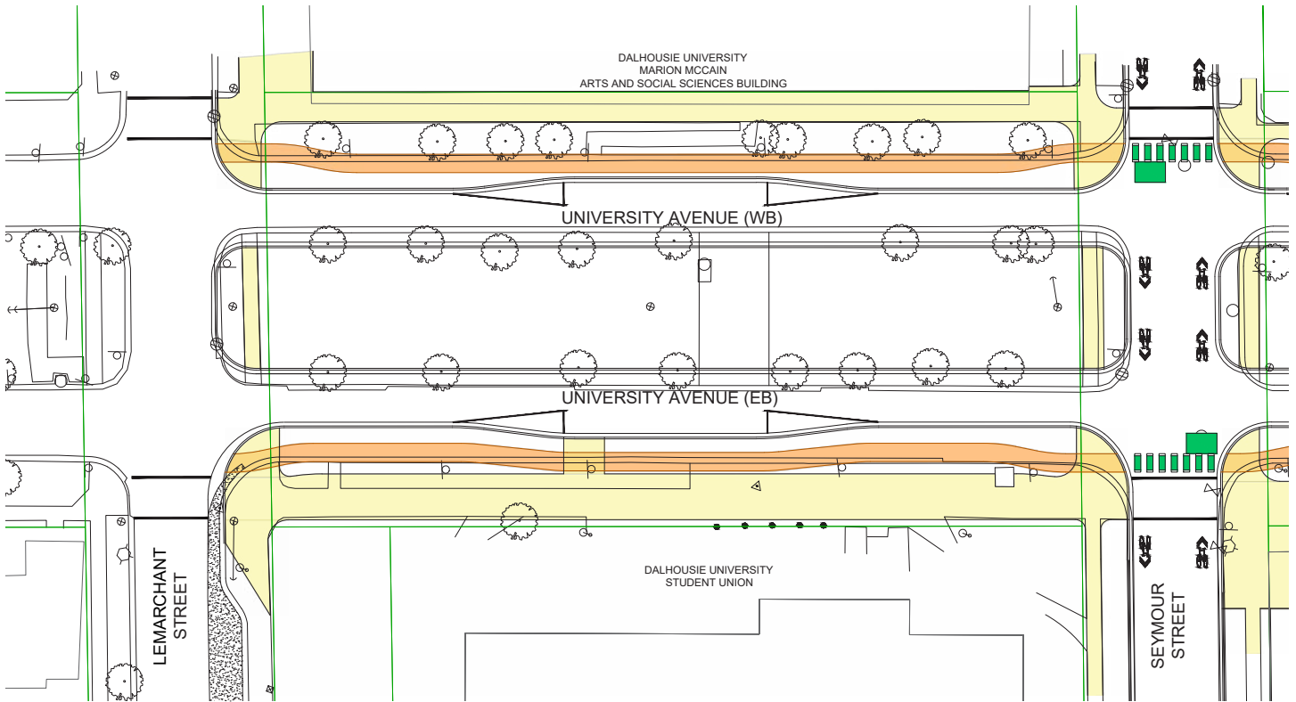
FUNCTIONAL DESIGN CONCEPT 2A One-Way Raised Bicycle Lanes
