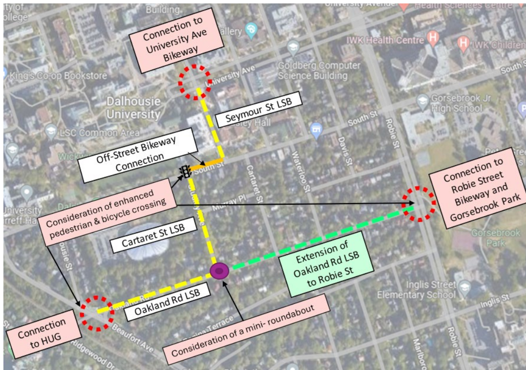
Figure 7: Seymour Street–Cartaret Street–Oakland Road Local Street Bikeway (Concept 3B)
