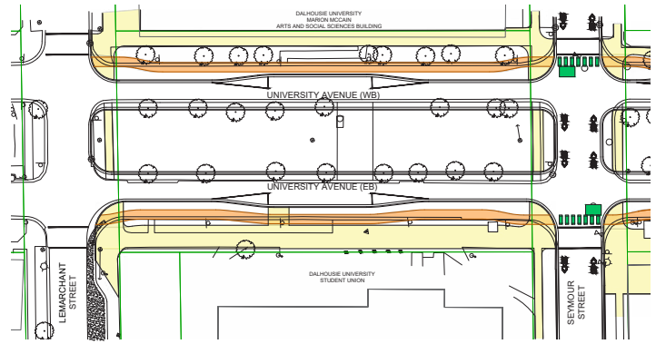
FUNCTIONAL DESIGN - CONCEPT 2A
