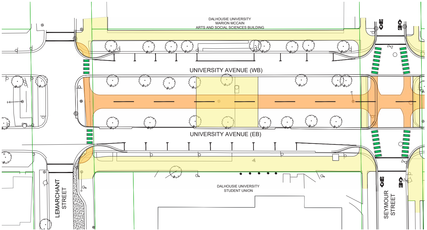
FUNCTIONAL DESIGN CONCEPT 2B Two-Way Bikeway in Median
