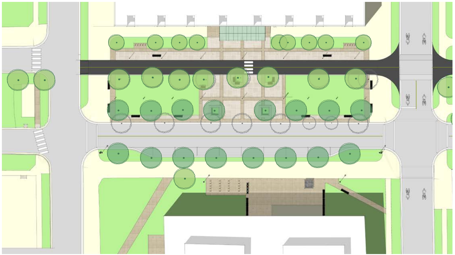
LANDSCAPE CONCEPT 2C Two-Way Bikeway North of Median
