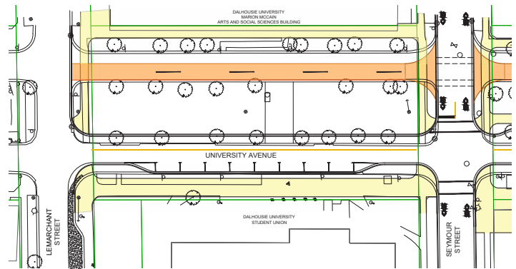
FUNCTIONAL DESIGN - CONCEPT 2C
