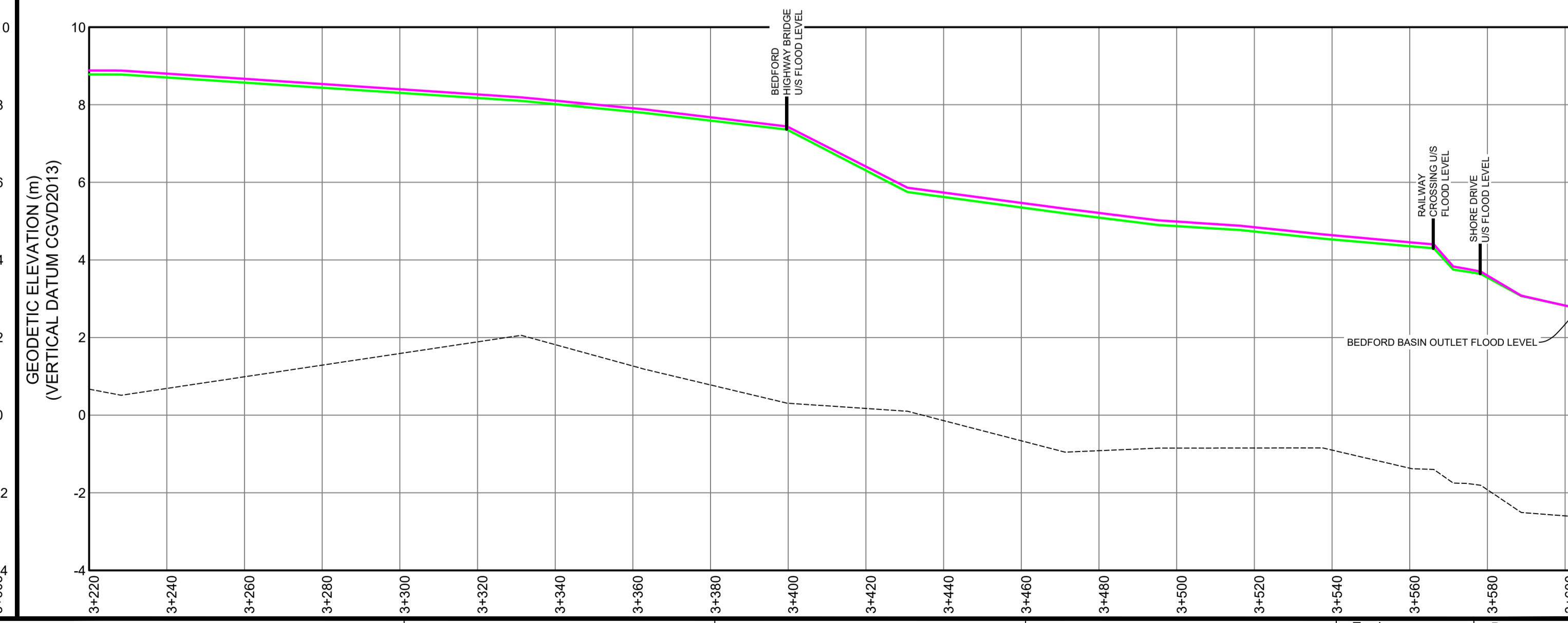
SACKVILLE RIVER APPROX. FLOOD LEVELS (1 IN 100 YEAR) - ADJACENT BEDFORD BASIN OUTLET SCALE: 1:1000 HORIZONTAL, 1:100 VERTICAL
