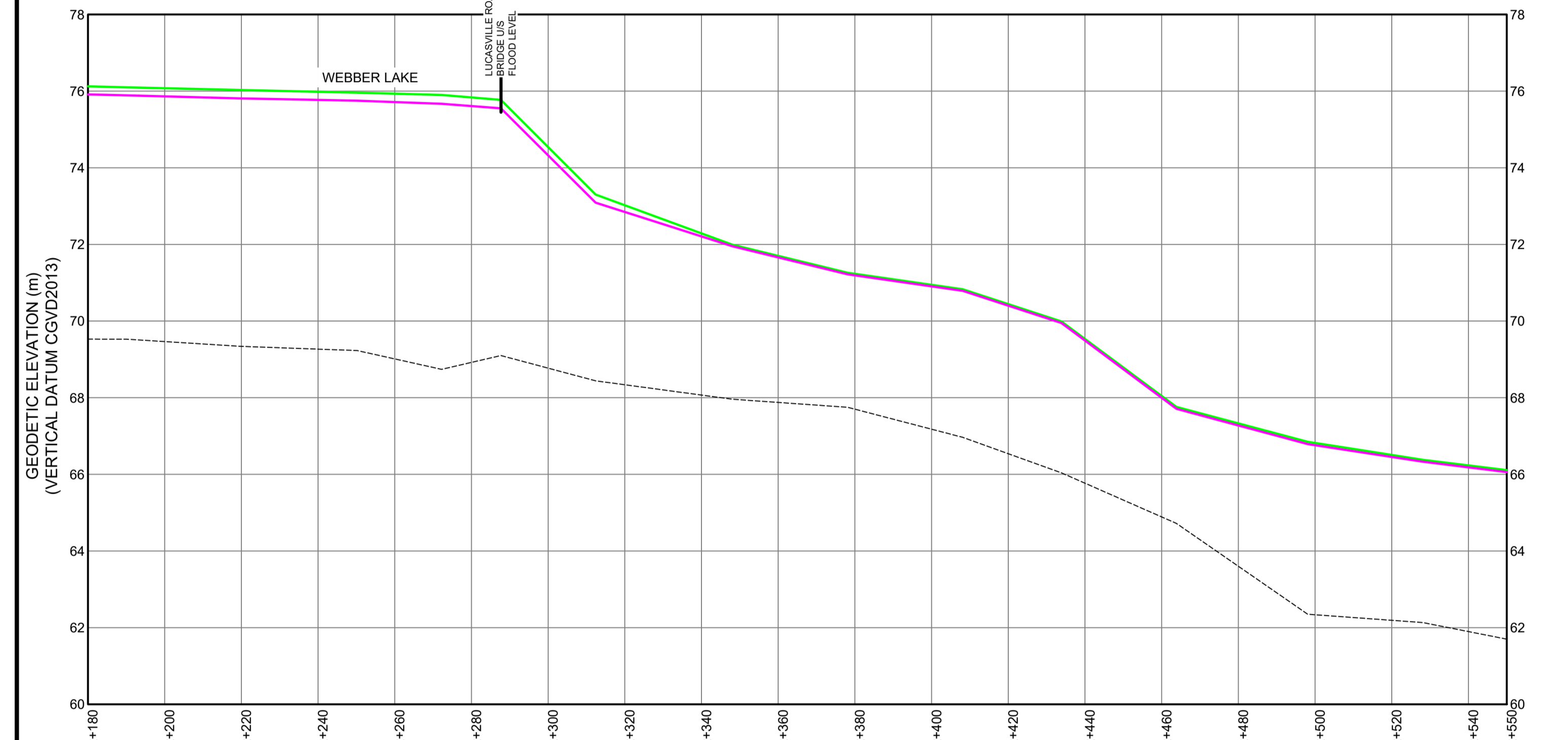
SACKVILLE RIVER APPROX. FLOOD LEVELS (1 IN 100 YEAR) - ADJACENT BEDFORD BASIN OUTLET SCALE: 1:1000 HORIZONTAL, 1:100 VERTICAL
