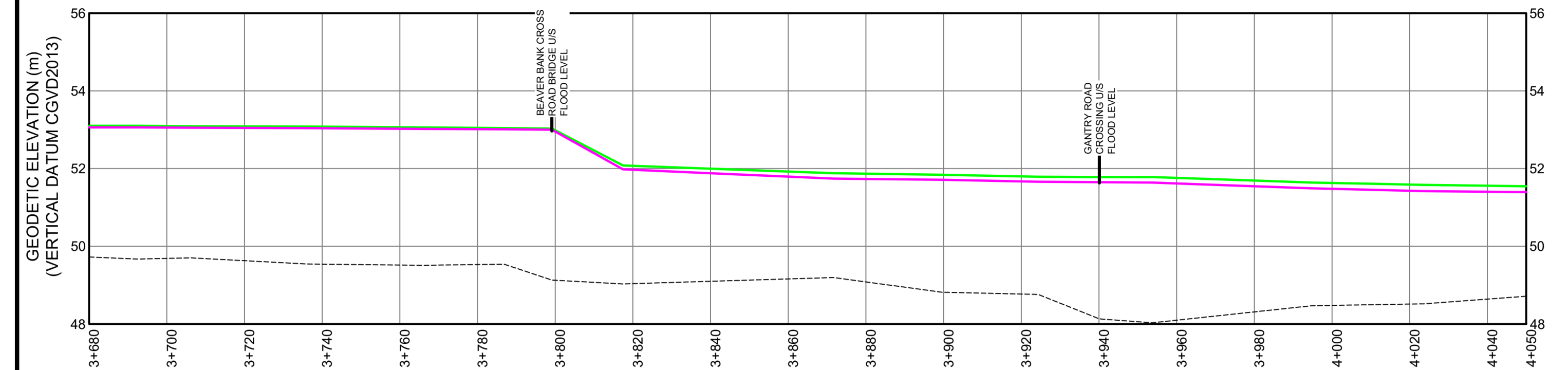
UPSTREAM SACKVILLE RIVER APPROX. FLOOD LEVELS (1 IN 100 YEAR) - ADJACENT LUCASVILLE RD. SCALE: 1:1000 HORIZONTAL, 1:100 VERTICAL
