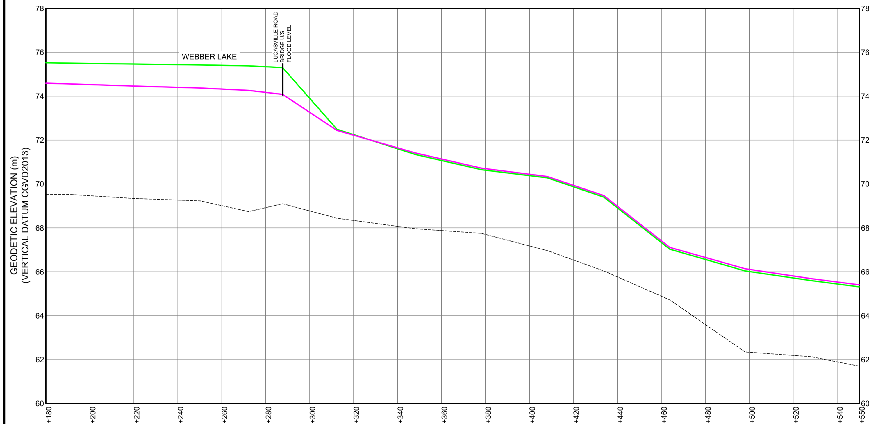
SACKVILLE RIVER APPROX. FLOOD LEVELS (1 IN 20 YEAR) - ADJACENT BEDFORD BASIN OUTLET SCALE: 1:1000 HORIZONTAL, 1:100 VERTICAL
