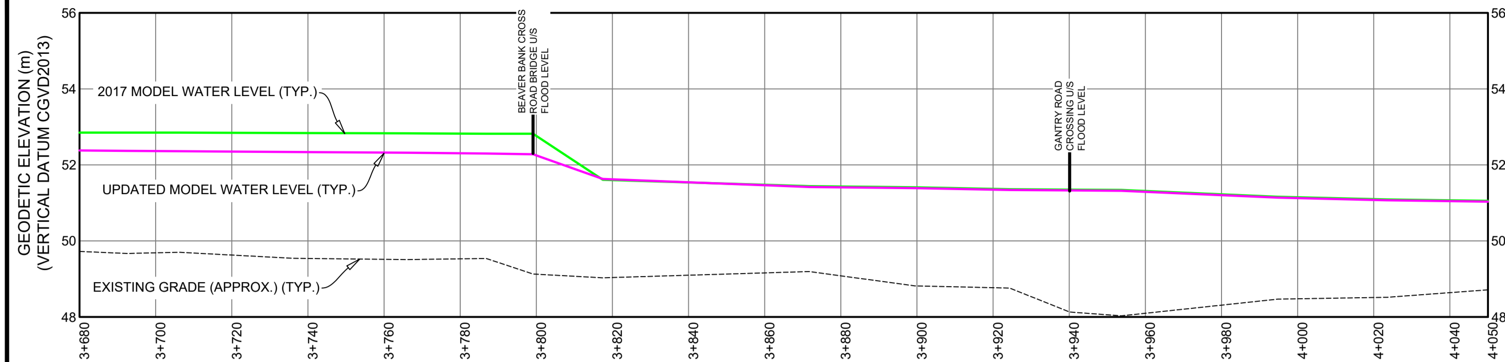
UPSTREAM SACKVILLE RIVER APPROX. FLOOD LEVELS (1 IN 20 YEAR) - ADJACENT LUCASVILLE RD. SCALE: 1:1000 HORIZONTAL, 1:100 VERTICAL
