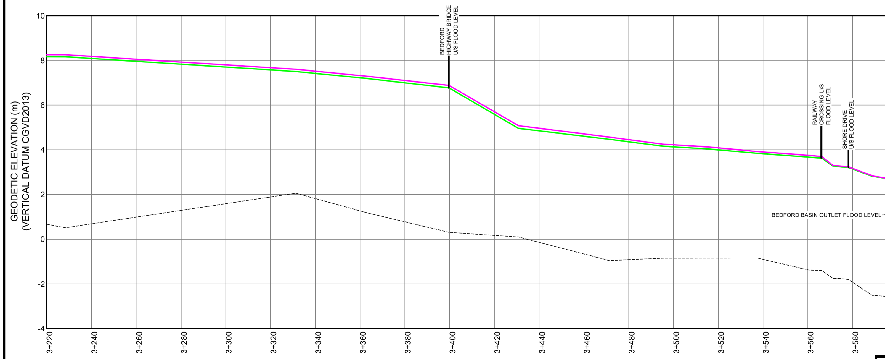
SACKVILLE RIVER APPROX. FLOOD LEVELS (1 IN 20 YEAR) - ADJACENT BEDFORD BASIN OUTLET SCALE: 1:1000 HORIZONTAL, 1:100 VERTICAL
