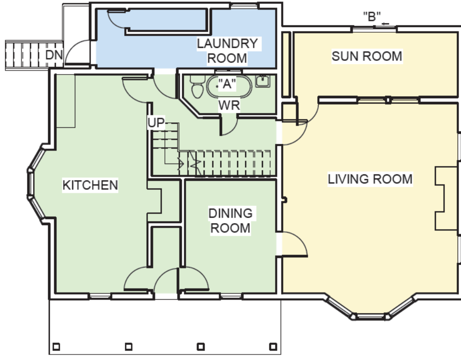
③ Level 1 3/32" = 1'-0"
