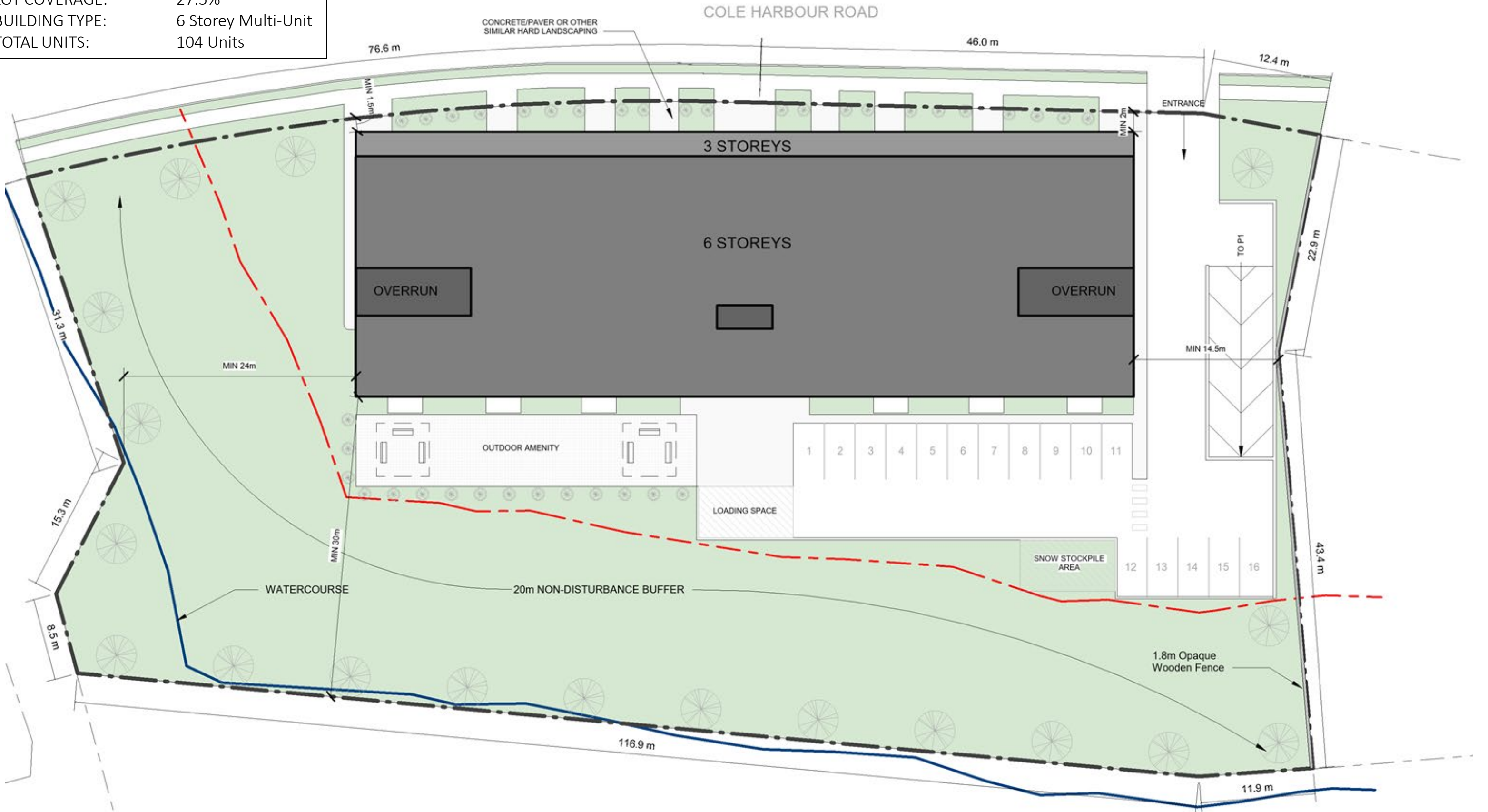
- SITE PLAN -
