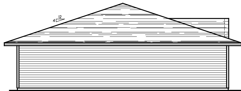
LEFT ELEVATION
