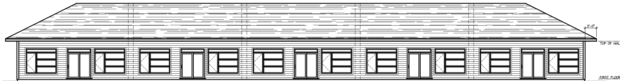
REAR ELEVATION
