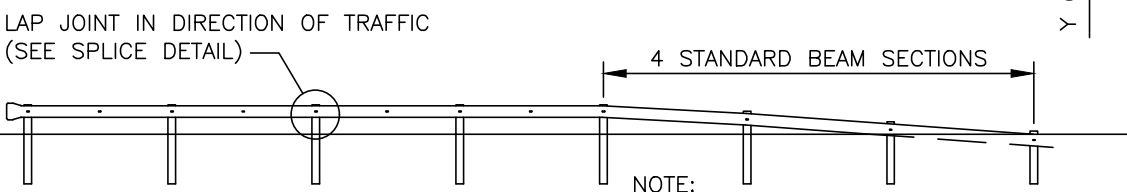
ELEVATION SCALE 1:200
