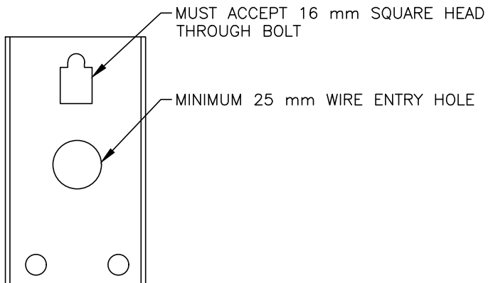
BRACKET
