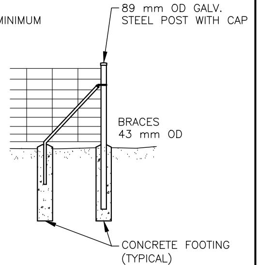
END OR CORNER POST AND BRACE SCALE: 1:60
