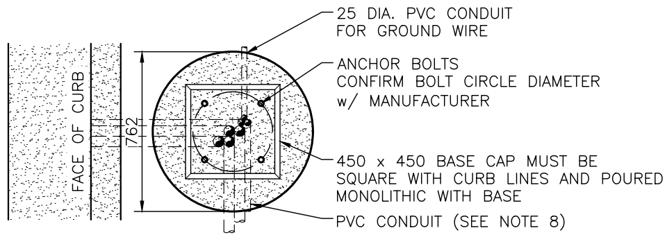
PLAN
