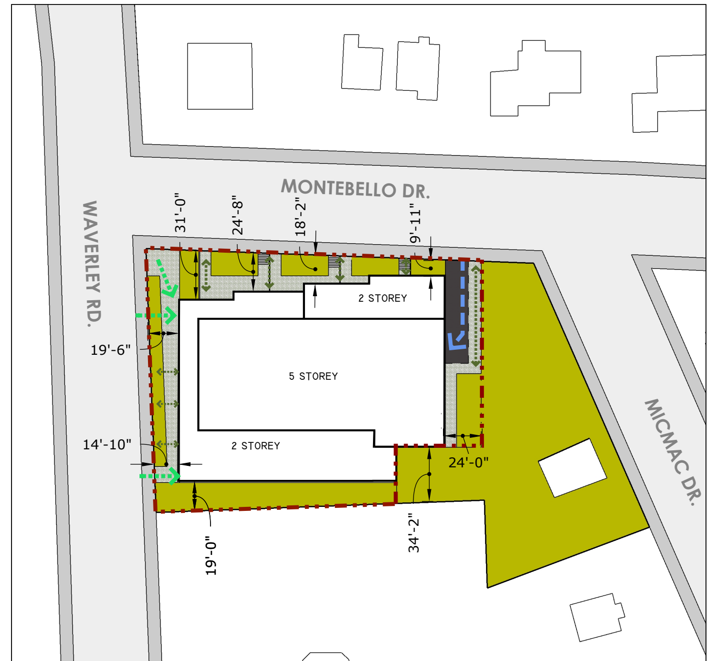
SITE PLAN
