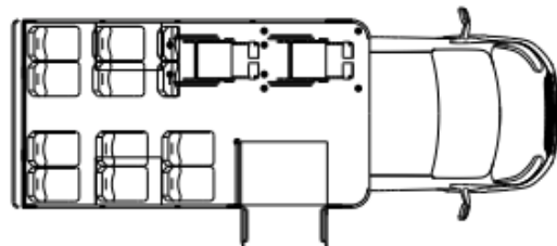
178" WB - 15 Passenger
