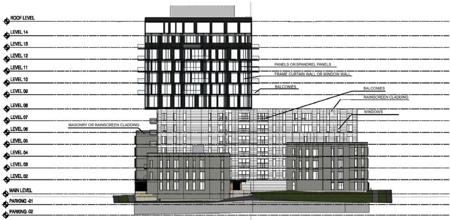
WEST ELEVATION 2018-04-18
