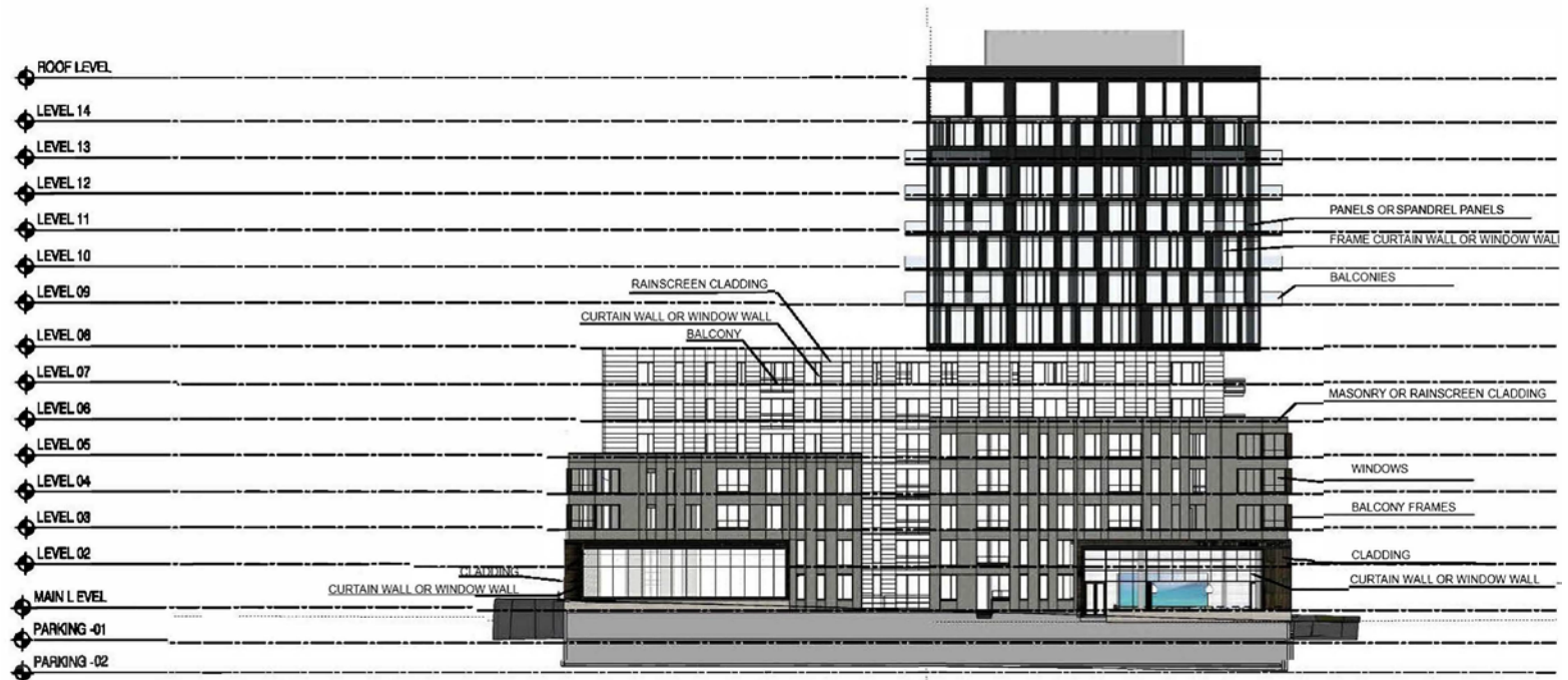
EAST ELEVATION 2018-04-18
